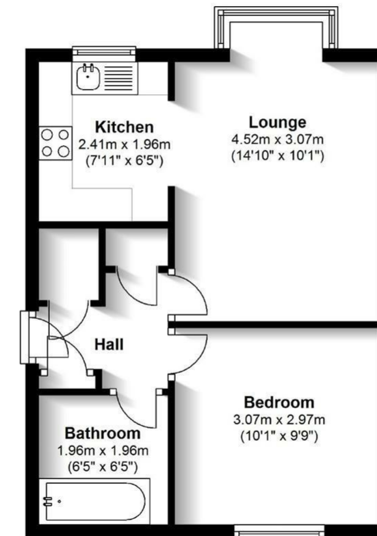
Ground Floor Approx. 36.7 sq. metres (394.8 sq. feet)
